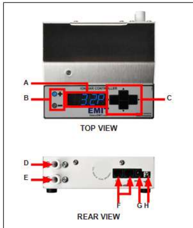
Figure 2. Pulsed Ion Bar Controller features and components
